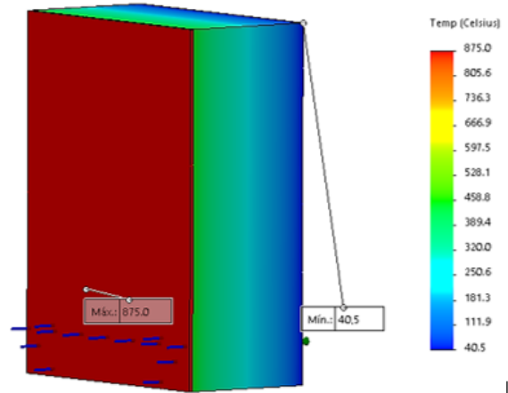
Fig. 2. Combustion room wall temperature simulation performed in thermal simulation by SolidWorks 2019 software.
