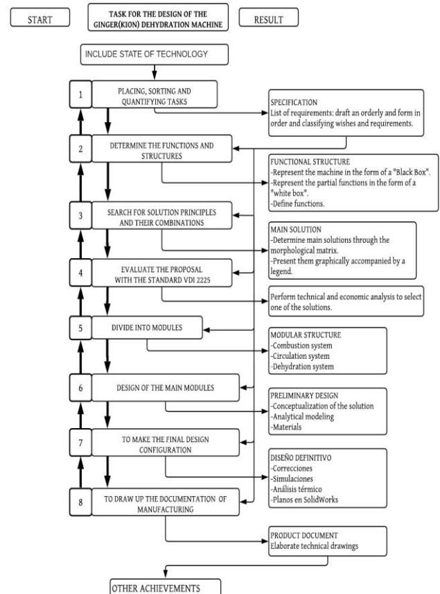
Fig. 2. Diagram of the design stages and processes adapting the design structure according to VDI 2221 complemented with VDI 2225 that develops the technical and economic analysis for the design of a forced internal convection dehydrator to improve ginger production.
