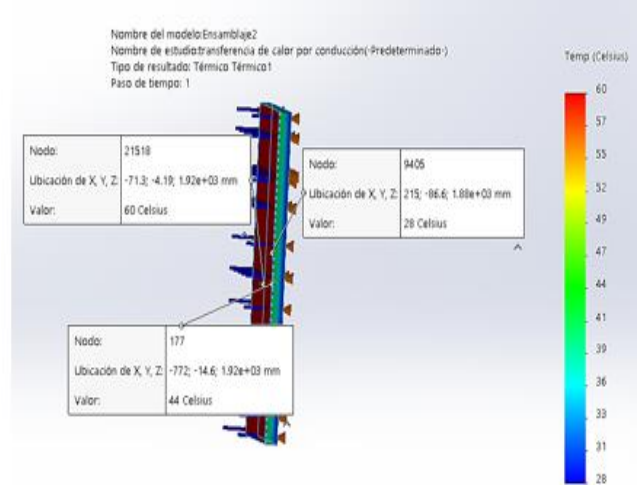
Fig. 5. Simulation of the temperature difference by walls elaborated in thermal analysis in SolidWorks 2019.
