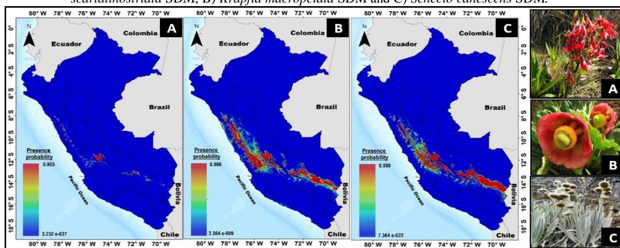
Figure 1. Model Specie Distribution for each specie with presence probability in Peru: A) Gentianella scarlatinostrata SDM, B) Krapfia macropetala SDM and C) Senecio canescens SDM.
