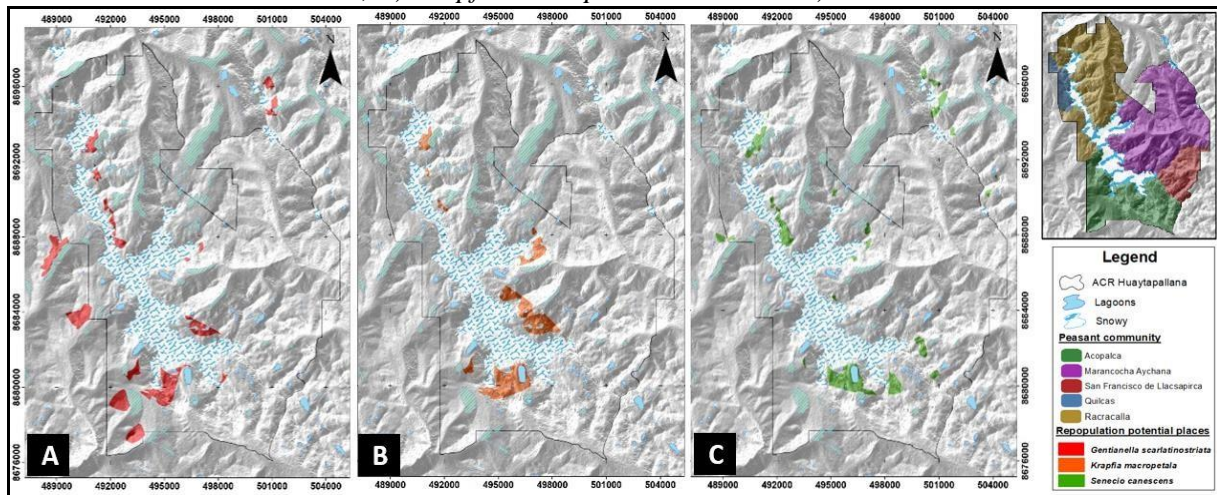
Figure 2. Repopulation potential model for each specie in the ACR-H: A) Gentianella scarlatinostrata model, B) Krapfia macropetala model and C) Senecio canescens model.
