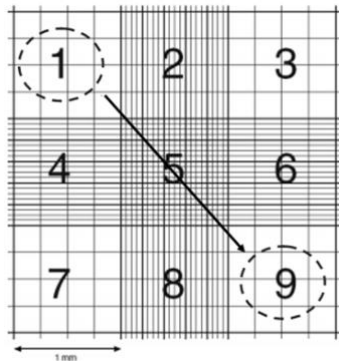
Fig. 4. Neubauer's chamber.
