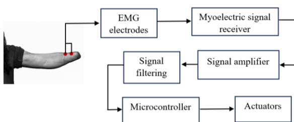
Fig. 8. Block diagram of EMG signal processing and control.
