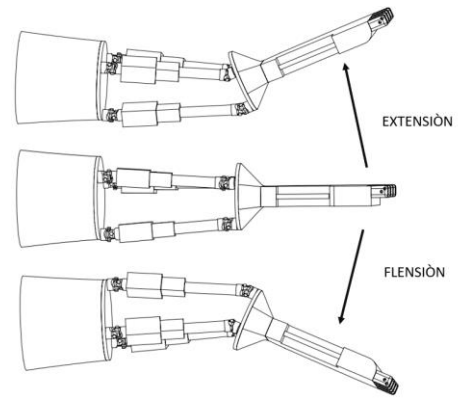
Fig. 12. Prototype wrist movement analysis (Flexion and Extension)
