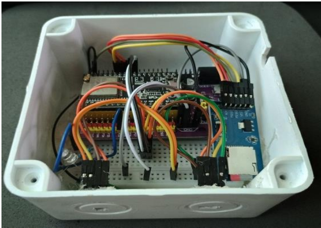
Fig. 5 Physical implementation of the ESP32-based system
