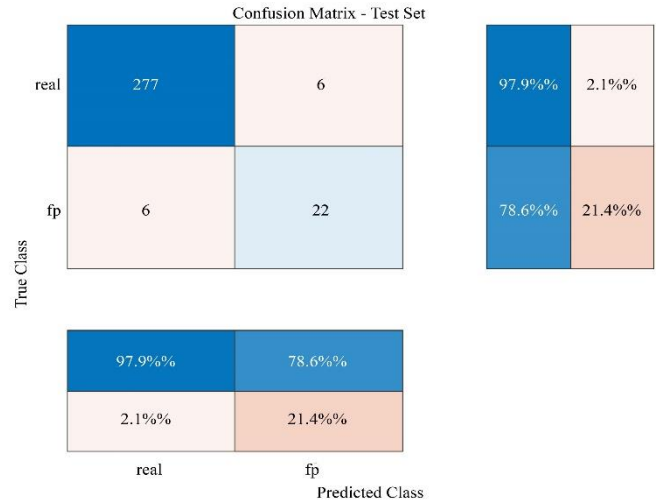
Fig. 12 Confusion matrix on the test set. Values are percentage-normalized by row
